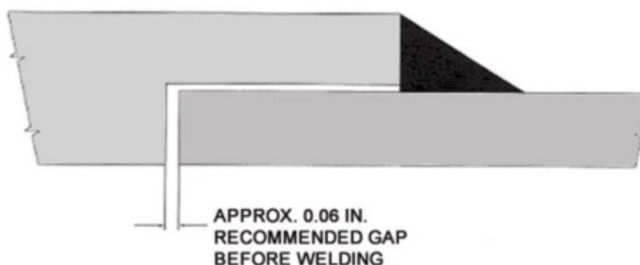
Figure 1 – Welding Gap
