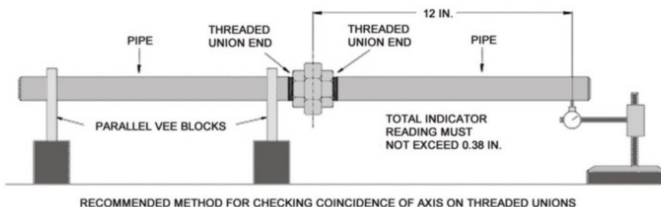
FIGURE 2 Recommended Method for Checking Coincidence of Axis on Threaded Unions (For Illustration Only)
